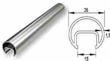
RAIL F-26 PARA CRISTAL DE Ø10 MM. Guide for glass / Code F50-305 / Weight 394 gr/m
