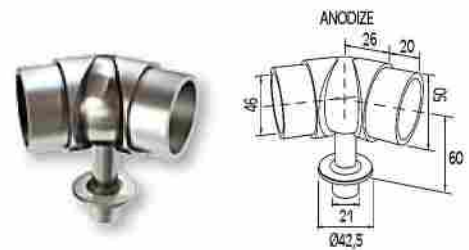
ARTICULACION ESQUINA F-50 Adjustable corner Ø50 railtop connector
