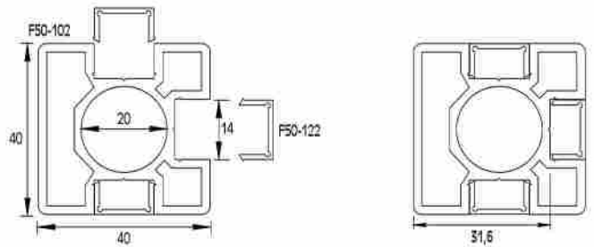
TAPA EMBELLECEDORA COLUMNA F50-102 Cover for F50-102 column / Code F50-122 / Weight 86 gr/m
