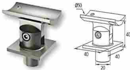
UNIÓN DE PASAMANOS A COLUMNA F50-102 Support for F50-200 handrail- F50-102 column (stairs) / Code 4356 / Pack. 50 /pcs.
