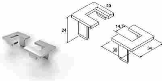
TAPA FINAL PERFIL F50-319 (PAR) End cap for F50-319 guide (perforated) / Code 4478 / Pack. 50 /pairs
