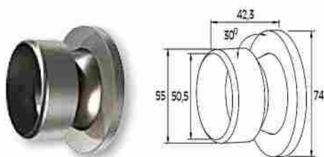
UNIÓN DE PASAMANOS PARED REGULABLE Wall cover for handrail Ø50 with cap / Code 4518 / Pack. 20 /pcs.
