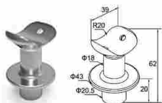
Support for handrail Ø40-column Ø42 (stairs)
