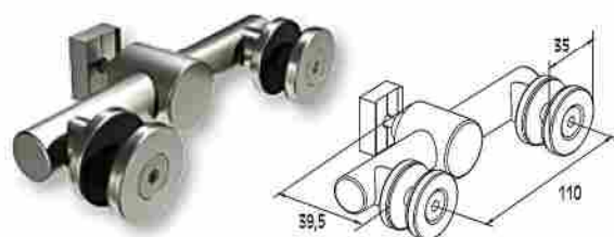
SOPORTE DOBLE PARA CRISTAL 8-10 MM Double glass support 8-10 mm for BLADE column
