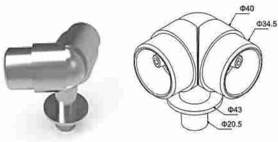
CONECTOR FLEXIBLE PARA PASAMNOS DE 40MM Adjustable corner connector for handrail Ø40 with column Ø42
