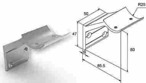
SOPORTE CONEXION PASAMANOS F50-200 A COLUMNA Fixed wall support for F50-200 handrail / Code 4134 / Pack. 20 /pcs.
