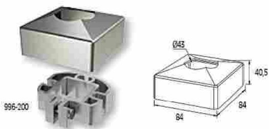
SOPORTE PARA COLUMNA DE 42 Support foot for Ø42 column / Code 4126 / Pack. 20 /pcs.
