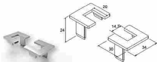
TAPA FINAL PERFIL F50-319 (PAR) End cap for F50-319 guide (perforated) / Code 4478 / Pack. 50 /pairs
