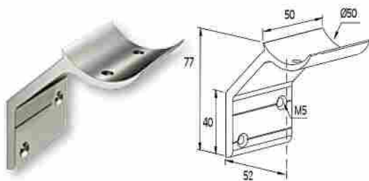
SOPORTE EXTERIOR PARA COLUMNA 40 X40 External support for 40x40 column / Code 4139 / Pack. 12 /pcs.
