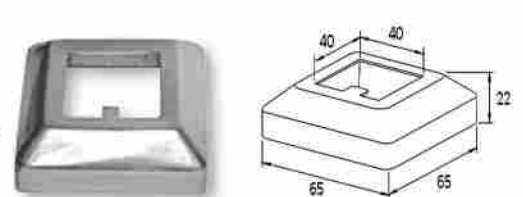
EMBELLECEDOR DE COLUMNA F50-102 Wall cover for F50-102 column / Code 4514 / Pack. 50 /pcs.
