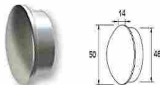
TAPA PASAMANOS F50-200 End cap for F50-200 handrail
