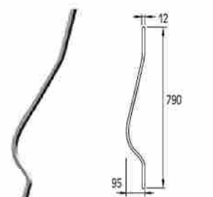
PERFIL CURVADO PARA VERTICAL-D Curved profile for Vertical-D / Code 4680 / Pack. 100 /pcs.
