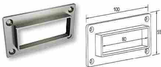
UNION PASAMANO A PARED F50-201, F50-203 Wall cover for F50-201/203 handrail / Code 4515 / Pack. 40 /pcs.
