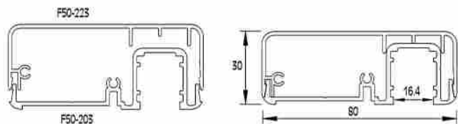
PASAMANOS DIVIDIDO 30 X 80 Cover for dividable handrail F50-203
