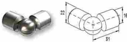
ARTICULACIÓN REGULABLE PARA RAIL F-16 Adjustable angle connector for profile Ø16
