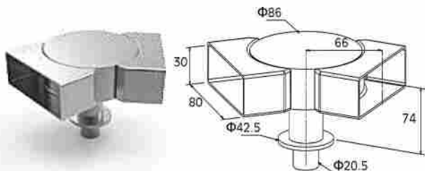
UNIÓN EN ESQUINA F50-201 CON F50-100 Adjustable corner connector for handrail 80x30 with column Ø42
