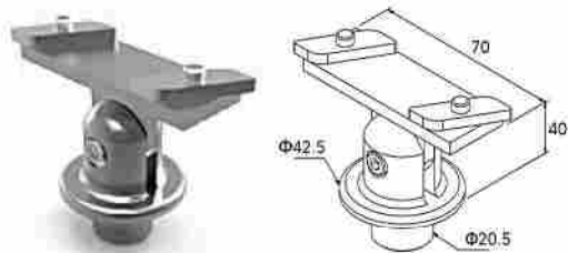
UNIÓN PASAMANOS F50-201 A F50-100 Support for F50-201 handrail-F50-100 column (stairs)
