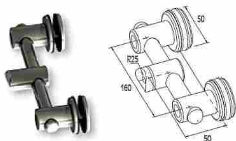
SOPORTE EXTERNO CRISTAL DOBLE DE 8-10 mm Double glass support 8-10 mm for Ø50 column
