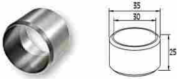
UNIÓN DE RAIL A RAIL Connector for guide Ø30 (straight) / Code 4242 / Pack. 20 /pcs.
