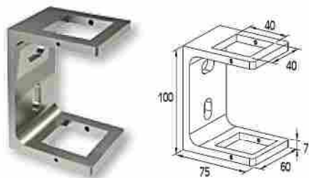
SOPORTE EXTERIOR PARA COLUMNA 40 X40 External support for 40x40 column / Code 4139 / Pack. 12 /pcs.
