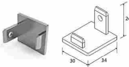
TAPA RAIL F50-319 End cap for F50-319 guide / Code 4477 / Pack. 40 /pcs.
