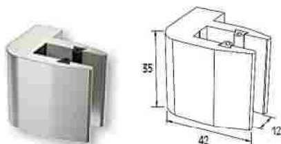
PINZA SENCILLA PARA CRISTAL 8-10mm COLUMNA F50-102 Single glass support 8-10 mm for F50-102 column
