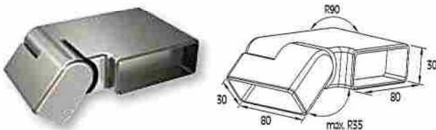
CONECTOR PARA PASAMANOS DE 80 X 30 Adjustable corner connector 90° for 80x30 handrail (stairs)
