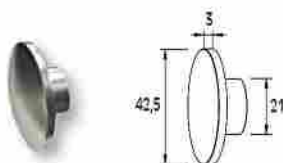
TAPA COLUMNA F50-100 End cap for F50-100 column
