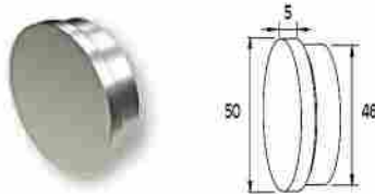
TAPA PASAMANOS F50-200 End cap for F50-200 handrail (flat) / Code 4453 / Pack. 50 /pcs.
