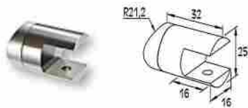
UNION COLUMNA F50-100 CON PERFIL F50-302 (16 x 16) Connector for F50-100 Column with F50-302 profile
