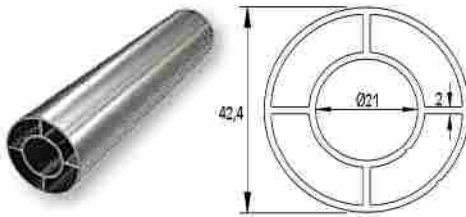
COLUMNA SUJECION Ø 42 mm Support column Ø42 / Code F50-100 / Weight 1025 gr/m
