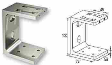
SOPORTE EXTERIOR PARA COLUMNA F50-108 External support for BLADE column / Code 4142 / Pack. 12 /pcs.
