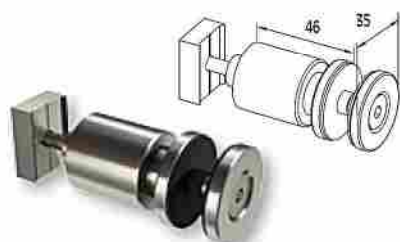
SOPORTE CRISTAL 8-10 MM PARA COLUMNA 4620 Single Glass support 8-10 mm for BLADE column / Code 4138 / Pack. 10 /pcs.
