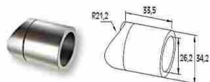
UNIÓN F50-100 CON PERFIL 26 MM Connector for F50-100 Column with profile Ø26 / Code 4252 / Pack. 50 /pcs.
