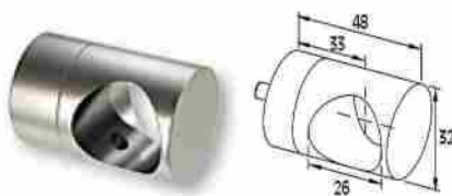
CONECTOR A COLUMNA F50-102 Connector for F50-102 column with profile Ø26 / Code 4358 / Pack. 50 /pcs.
