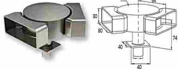
UNIÓN EN ESQUINA DE 80 X 30 DE PASAMANOS A COLUMNA Adjustable corner connector for 80x30 handrail with F50-102 column / Code 4357 / Pack. 2 /pcs.
