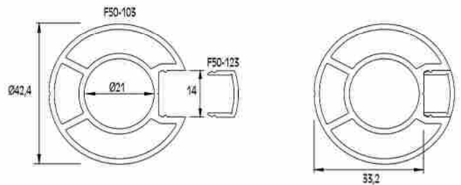
TAPA EMBELLECEDORA DE COLUMNA F50-103 Cover for F50-103 column / Code F50-123 / Weight 90 gr/m
