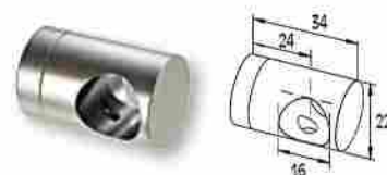
CONECTOR DE 16 A COLUMNA F50-102 Connector for F50-102 column with profile Ø16 / Code 4359 / Pack. 50 /pcs.
