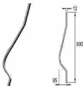
PERFIL CURVADO PARA VERTICAL-D Curved profile for Vertical-D / Code 4670 / Pack. 100 /pcs.
