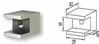
UNION EXTERNA DEL PERFIL F50-102/106 Y PERFIL F50-302 Connector for F50-102/106 Column with F50-302 profile / Code 4245 / Pack. 100 /pcs.
