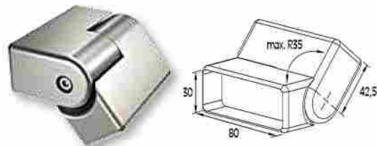
CONECTOR PARA PASAMANOS DE 80 X 30 Adjustable corner connector for 80x30 handrail (stairs)
