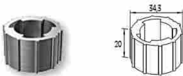
ROSETA 20 MM PARA COLUMNA F50-104 COLOR BRUTO Adaptor for F50-104 Column / Code 4248 / Pack. 50 /pcs.
