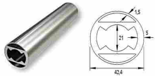
COLUMNA DE 42 MM Support column Ø42 (heavy-duty)
