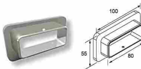
TAPA UNIÓN PARED Wall cover for F50-201/203 handrail (with cap) / Code 4515Z / Pack. 40 /pcs.
