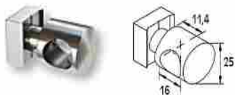
UNION DE COLUMNA 4620 PARA F-16 Connector for profile Ø16 with BLADE column
