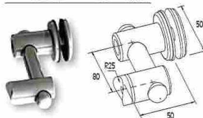
SOPORTE BÁSICO DE CRISTAL EXTERNO A COLUMNA Single glass support 8-10 mm for Ø50 column
