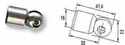
UNIÓN ROSETA CRISTAL CON F-16 Connector for glass rosette with profile Ø16
