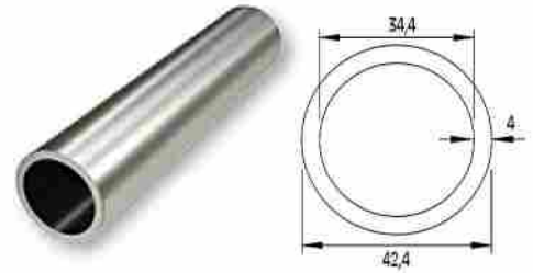
COLUMNA DE 42 MM. Support column Ø42 / Code F50-104 / Weight 1303 gr/m
