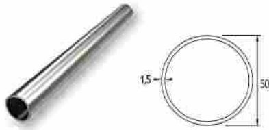
PASAMANOS F-50 (Ø50mm), GROSOR 1,5 Handrail Ø50 / Code F50-205 / Weight 617 gr/m
