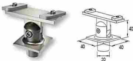
UNION DE COLUMNA 4620 PARA F-16 Connector for F50-102 column with F50-201 handrail
