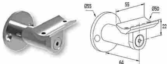
SOPORTE A PARED PARA PASAMANOS F50-200 Wall support for F50-200 handrail / Code 4140 / Pack. 20 /pcs.
