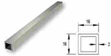
RAIL CUADRADO 16 X 16 X 2 MM Square 16x16x2 / Code F50-302 / Weight 302 gr/m
