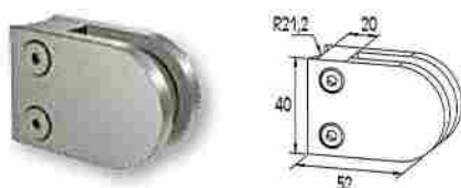
PINZA DE SUJECCION 6-8 MM INOX Glass support 6-8 mm
