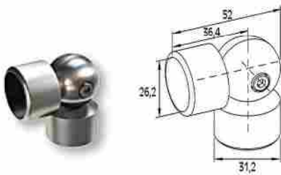
PERFIL CONECTOR DE 26MM Adjustable corner connector for profile Ø26 / Code 4352 / Pack. 20 /pcs.
