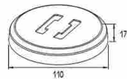
PIE PARA COLUMNA F50-108 F50-108 Column support foot
