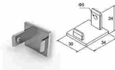
TAPA RAIL F50-319 End cap for F50-319 guide / Code 4477 / Pack. 50 /pcs.
