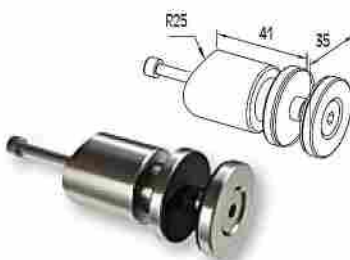
SOPORTE CRISTAL 8-10 MM PARA COLUMNA F50-100 Glass support 8-10mm for F50-101 column / Code 4137 / Pack. 10 /pcs.
