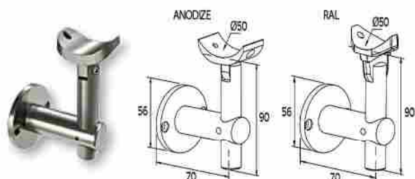
UNIÓN PARED PASAMANOS F50-200 Wall support for F50-200 handrail
