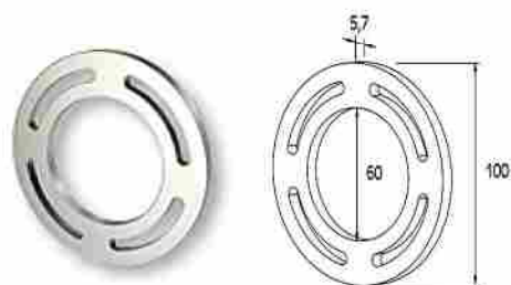
ROSETA DECORATIVA CRISTAL Glass rosette Ø100 / Code 4611 / Pack. 20 /pcs.
