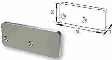
TAPA PASAMANOS F50-203 End cap for F50-203 handrail / Code 4451 / Pack. 10 /pair
