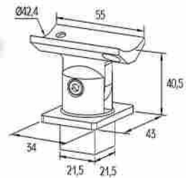
UNION COLUMNA CON PASAMANOS DE 42MM Ø42 Railtop support stairs
