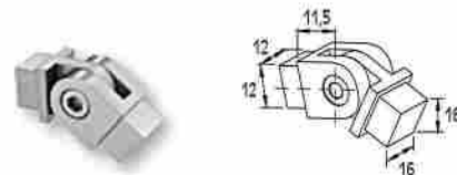
UNION EN ESQUINA DE RAIL F50-302 (16 x 16) Adjustable corner connector for F50-302 profile
