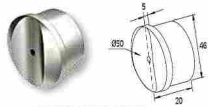
CONECTOR DE PASAMANOS F50-200 (CONECTOR VERTICAL) Connector for handrail with handrail F50-200
