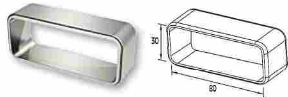
UNION DE PASAMANOS 80 x 30mm Connector for 80x30 handrails straight / Code 4249 / Pack. 20 /pcs.
