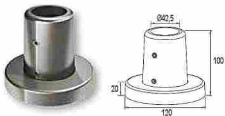
SOPORTE REFORZADO PARA COLUMNA DE 42 Heavy duty support foot for Ø42 column / Code 4127 / Pack. 20 /pcs.
