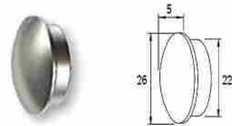
TAPA PERFIL F50-304 End cap for F50-304 profile / Code 4461 / Pack. 50 /pcs.
