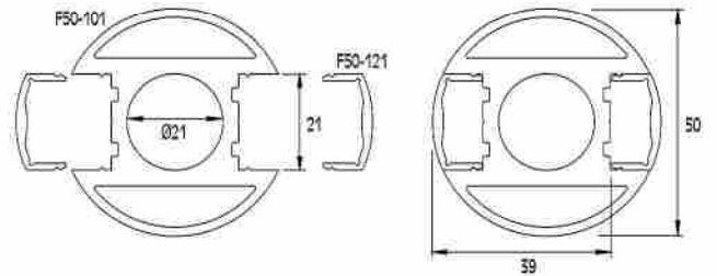
TAPA EMBELLECEDORA DE COLUMNA Cover for F50-101 column / Code F50-121 / Weight 152 gr/m
