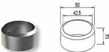
EMBELLECEDOR COLUMNA F50-100 Wall cover for column Ø42 / Code 4510 / Pack. 50 /pcs.
