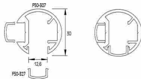
TAPA EMBELLECEDORA DE F50-307 Rail cover
