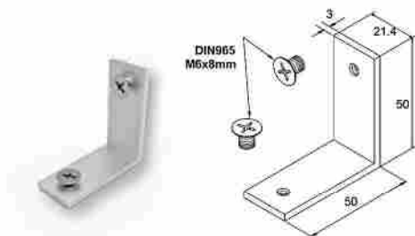
CONECTOR PARA LA GUIA F50-319 Connector for F50-319 guide / Code 4259 / Pack. 50 /pcs.
