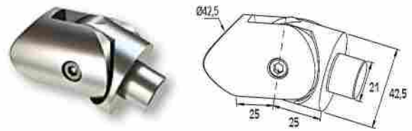
CONECTOR F50-100 EN ESCALERA Connector for column with column F50-100 (stairs) / Code 4355 / Pack. 30 /pcs.
