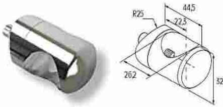
CONECTOR COLUMNA F50-101 PARA PERFIL DE 26MM Connector for F50-101 column with profile Ø26 / Code 4348B / Pack. 50 /pcs.
