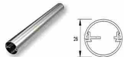
RAIL ESPECIAL Ø26 MM PARA F50-303 AGUJERADO Perforated Ø26 guide for F50-303 profile / Code F50-306 / Weight 368 gr/m
