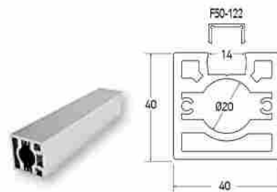
SOPORTE DE COLUMNA 40 X 40 Support column 40x40 (without cap)
