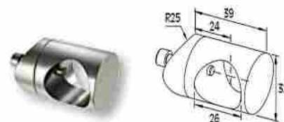
CONECTOR COLUMNA F50-101 PARA PERFIL DE 26MM Connector for F50-101 column with profile Ø26
