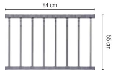
COD. 42-02 MOD. LINEAL
