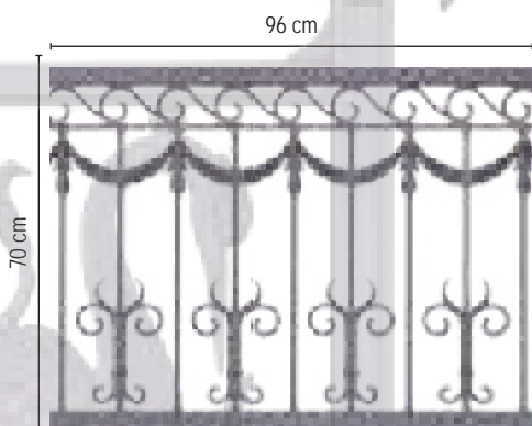
COD. 70-26 MOD. GIRNALDA
